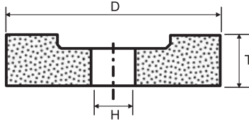
TYPE 5
