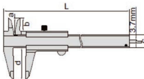
1205-150S Shown
