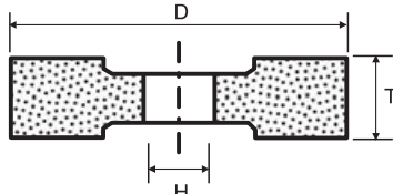
TYPE 7
