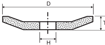
TYPE 12
