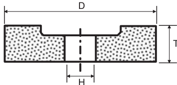
TYPE 7
